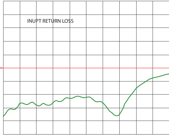
CH1 S11 log MAG 5 dB/ Ref -20dB
