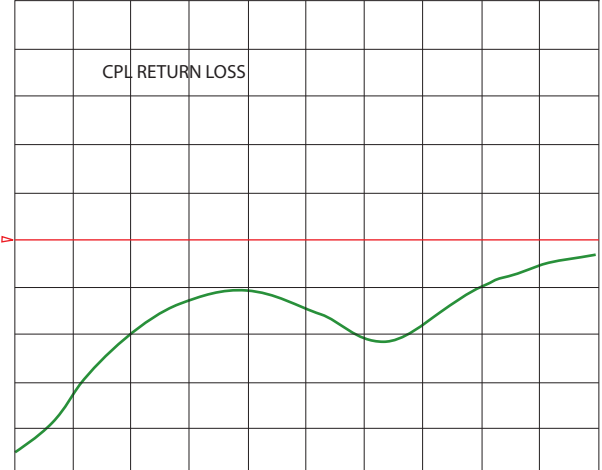
CH1 S33 log MAG 5 dB/ Ref -17.8 dB
