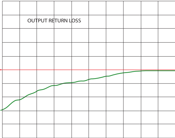
CH1 S22 log MAG 5 dB/ Ref -17.8 dB
